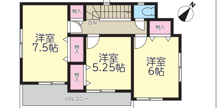
2階平面図:43.89㎡(13.27坪)
